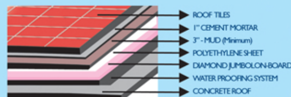
ROOF INSULATION Method - 1
