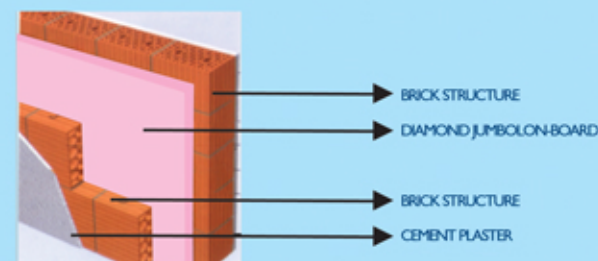
WALL INSULATION
